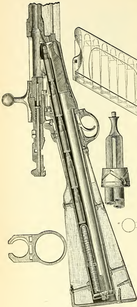
The Mannlicher Revolving Magazine Repeater.
